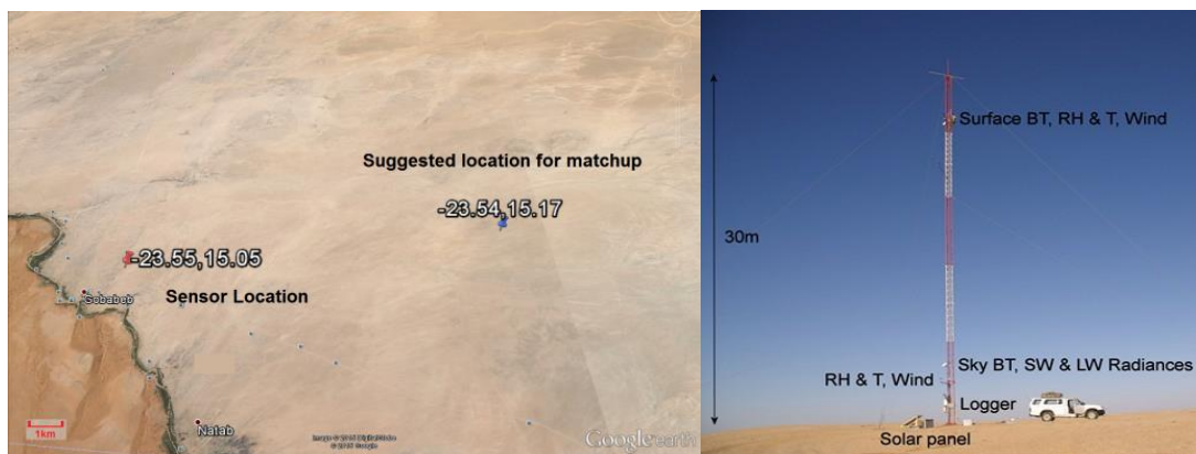
Figure 2-25 (a) is Geographic landscape in Gobabeb station in Namibia and (b) is the instrumentation for LST measurement: two radiometers measure the surface-leaving radiance (9.6–11.5 \mu\text{m} ) from the gravel plain, which is highly homogenous over at least 2500 \text{km}^2 .
