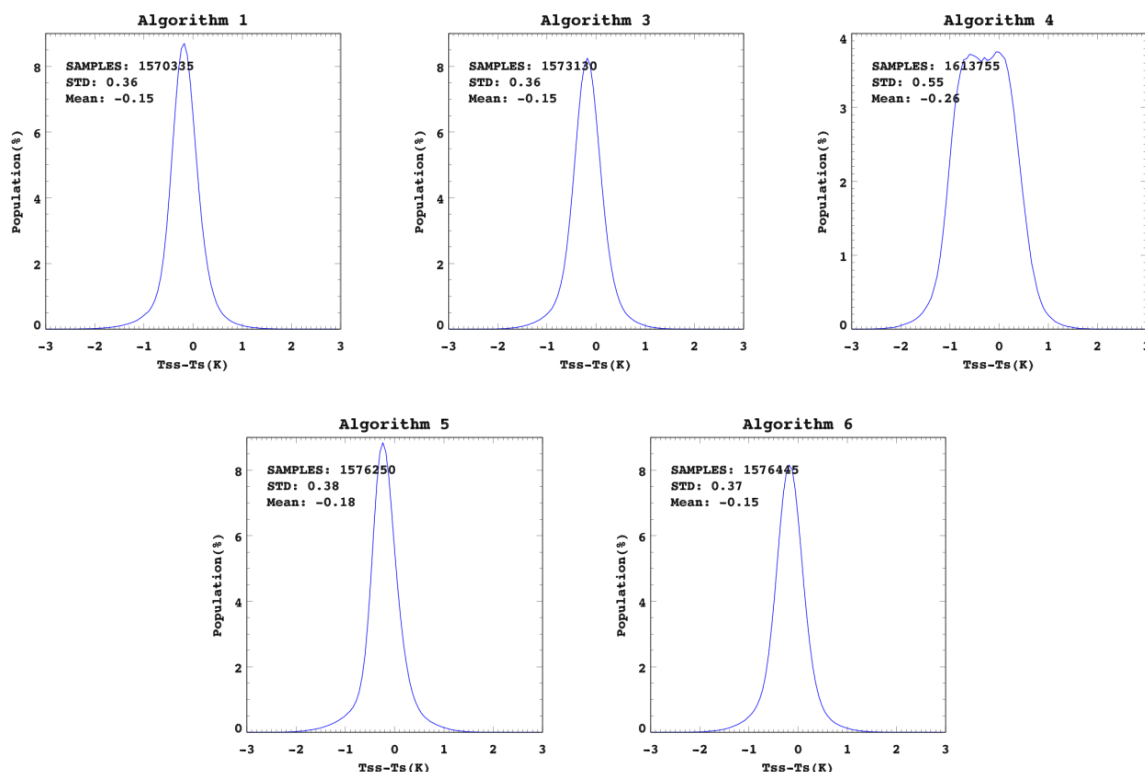
Figure 2-10 Histogram plots of the regression results for the dry atmosphere (tpw: 0.0-1.5 at Daytime). Standard deviation (STD) and mean errors of the regression are given in each plot.
