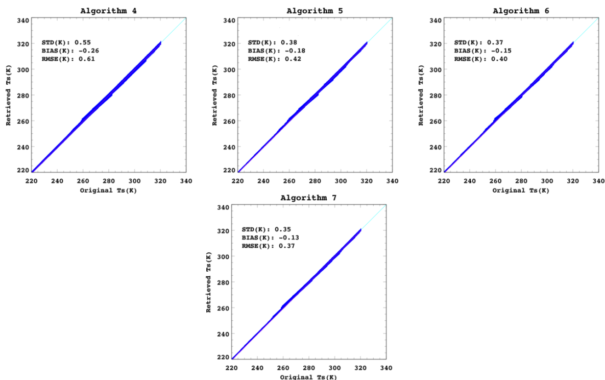
Figure 2-9 Scatter plots of the regression results for the dry atmosphere. Standard deviation (STD) errors of the regression are given in each plot (Daytime).
