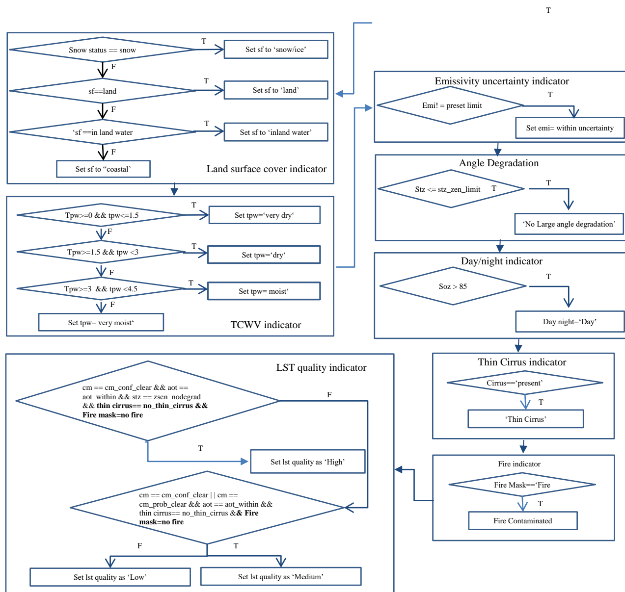
Figure 2-8 Flow chart for quality flag settings
