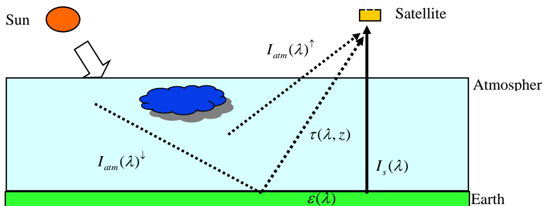
Figure 2-3 Radiation components reached to satellite sensor.
