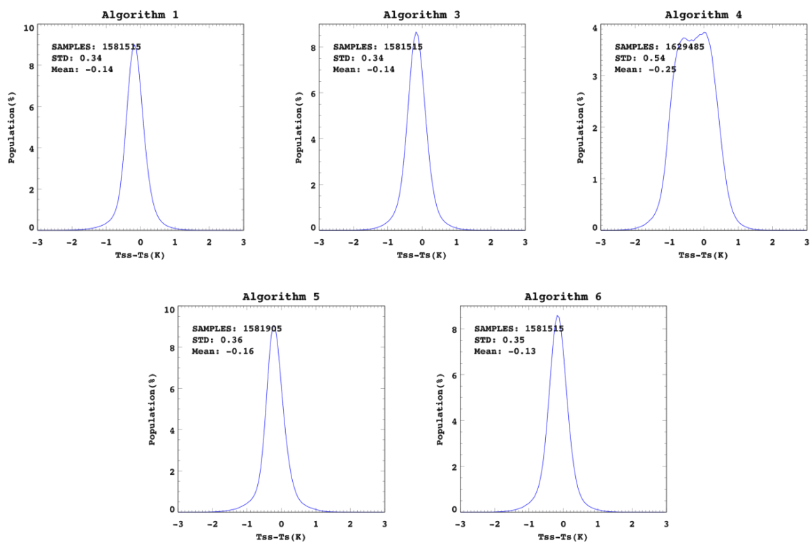
Figure 2-13 Histogram plots of the regression results for the dry atmosphere ( T_{pw} : 0.0-1.5 at Nighttime). Standard deviation (STD) and mean errors of the regression are given in each plot.
