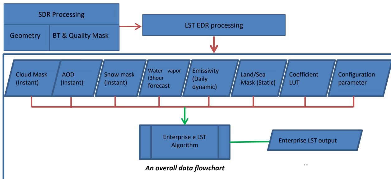
Figure 2-1 High level data flow of the enterprise LST algorithm.
